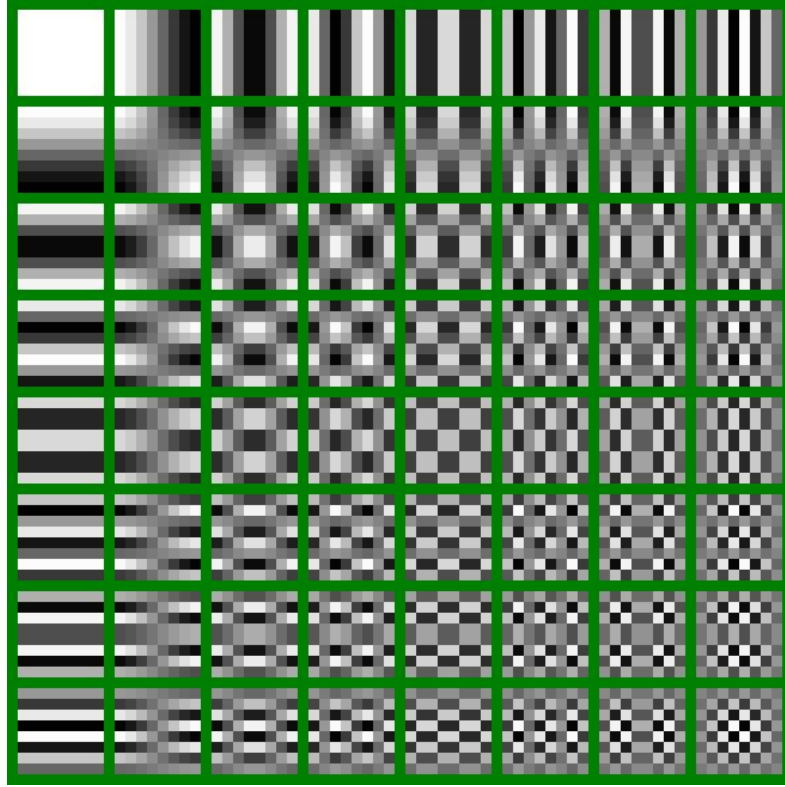
Figure 3. 2D basis functions for N = 8 .
