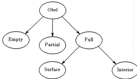
Figure 1: Types of Octree Obels
